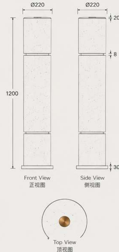
Brass Touch Control 黄铜触控件 Ø20 mm | Matte Finish
